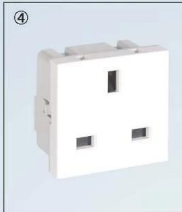
③ XJY-QB-29 Universal socket Rated voltage: 250v Rated current: 10a Size: 45*45mm Color: White Material: PC
