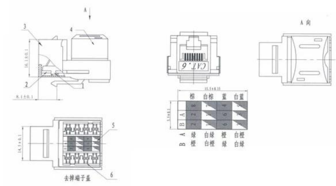
Cat6 Drawing:
